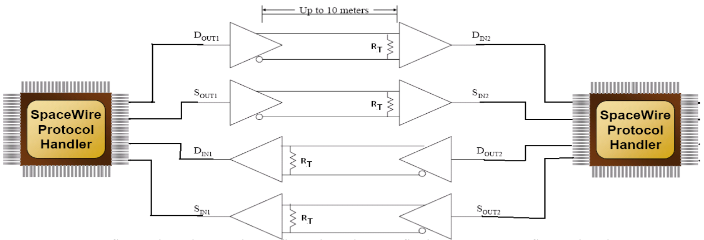
SpaceWire point-to-point configuration using LVDS. Diagram shows one SpaceWire Link
